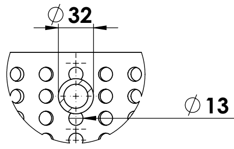
DETAIL B SCALE 2 : 7
